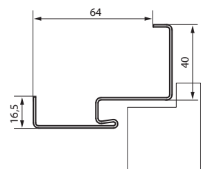
DOOR FRAME CROSS-SECTION
